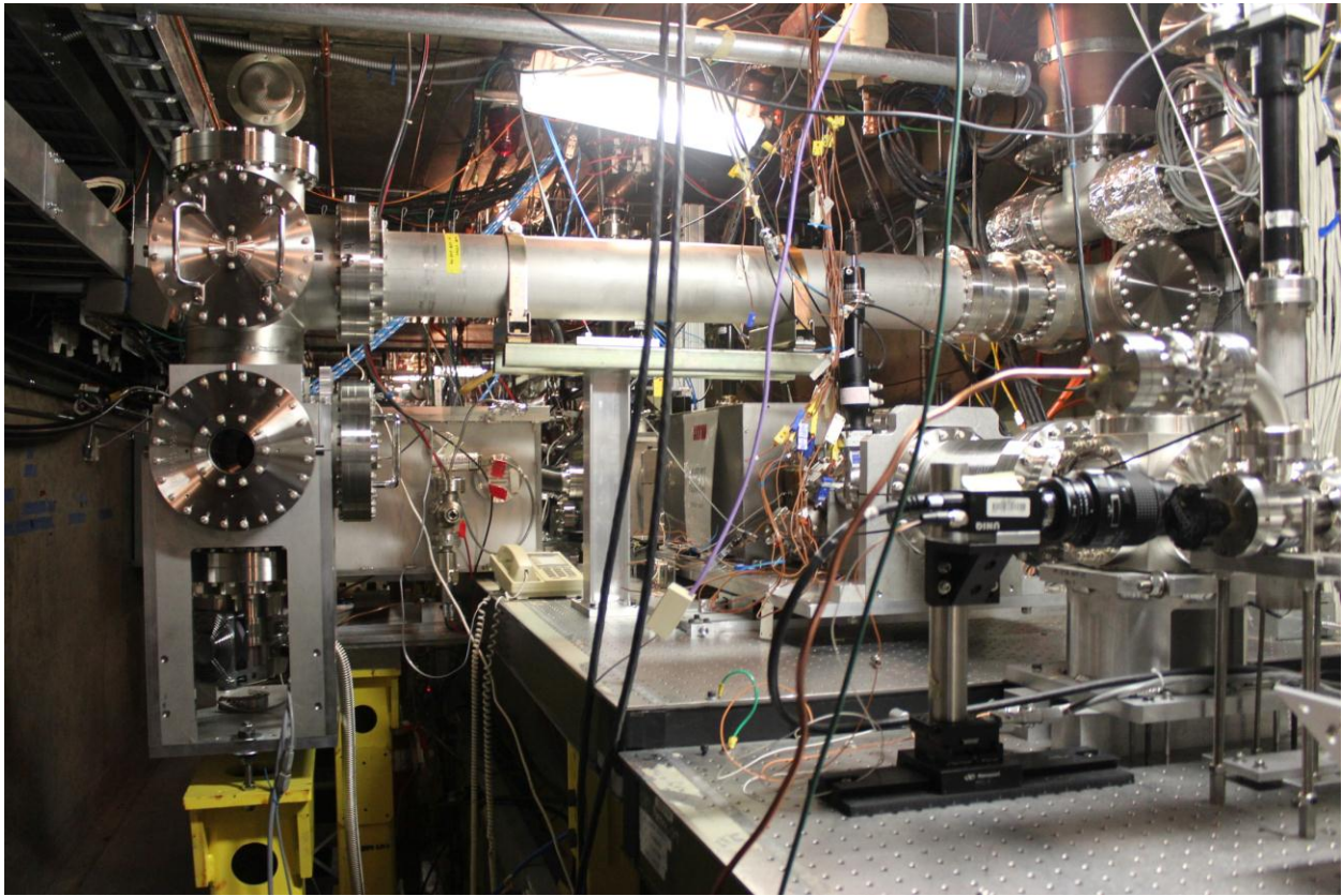
Figure 1: Laser Transport line in the tunnel is installed along with the compressor box and a chamber for integration with the FACET beamline.
