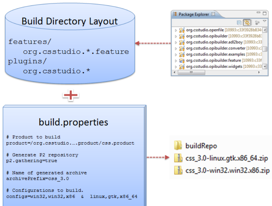
Figure 4.6. Headless Build
