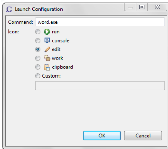
Figure 32.2. Configuration Editor
