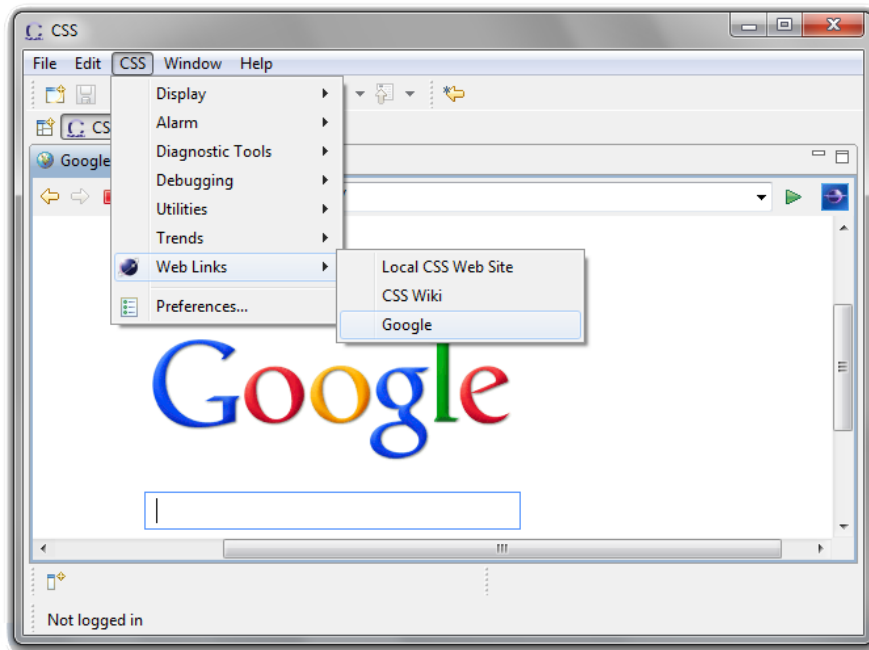
Figure 34.1. Web menu
